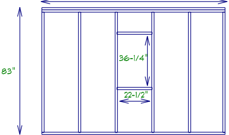
Left Gable Wall Layout
