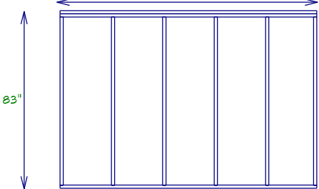
Right Gable Wall Layout
