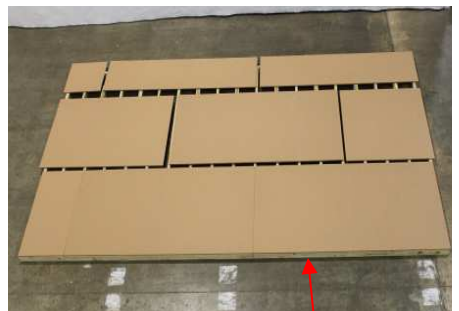
(33) Nail the rest of the first row, then move to next step.
