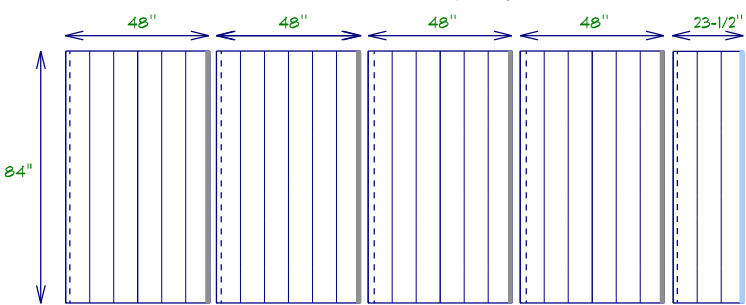
Back Wall Siding Layout
