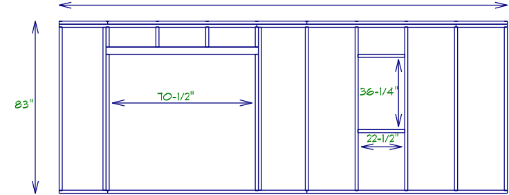
Front Wall Layout (Doors aligned to the left)
